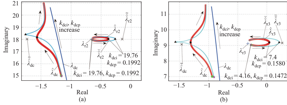
Fig. 8. Trajectories of eigenvalues and their estimates as k_{dcp} and k_{dci} increase from k_{dcp} = 0.1472 , k_{dci} = 4.16 to k_{dcp} = 0.2621 , k_{dci} = 38.63 . (a) Displays the trajectories of \lambda_{r2} , \hat{\lambda}_{r2} , \lambda_{dc} and \hat{\lambda}_{dc} as k_{dcp} and k_{dci} are tuned from k_{dcp} = 0.1992 , k_{dci} = 19.76 to k_{dcp} = 0.2621 , k_{dci} = 38.63 . (b) The trajectories of \hat{\lambda}_{r3} , \lambda_{dc} and \hat{\lambda}_{dc} , as well as the location of \lambda_{r3} with both k_{dcp} and k_{dci} increasing from k_{dcp} = 0.1472 , k_{dci} = 4.16 to k_{dcp} = 0.1739 , k_{dci} = 12.17 .
