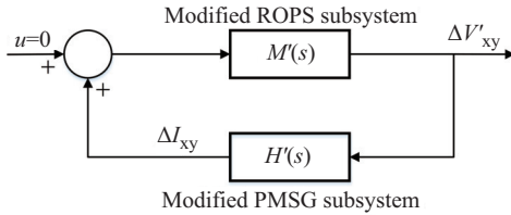
Fig. 3. Closed-loop model for calculation of residue of open-loop modes of ROPS subsystem.
