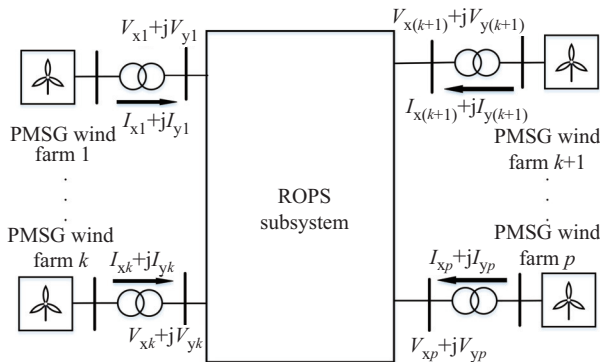
Fig. 1. A multi-machine power system with p PMSG wind farms.
