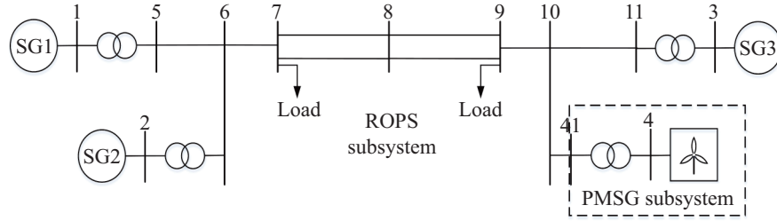
Fig. 7. Configuration of the 4-machine 11-bus power system.
