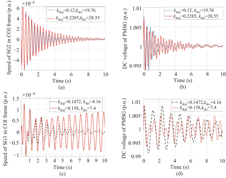
Fig. 9. Results of time domain simulation on the 4-machine 11-bus power system. (a) The difference between the speed of SG2 when control parameter k_{dcp} = 0.12, k_{dci} = 19.76 and k_{dcp} = 0.2285, k_{dci} = 28.55 . (b) The difference between the DC voltage of PMSG when control parameter k_{dcp} = 0.12, k_{dci} = 19.76 and k_{dcp} = 0.2285, k_{dci} = 28.55 . (c) The difference between the speed of SG3 when control parameter k_{dcp} = 0.1472, k_{dci} = 4.16 and k_{dcp} = 0.158, k_{dci} = 7.4 . (d) The difference between the DC voltage of PMSG when control parameter k_{dcp} = 0.1472, k_{dci} = 4.16 and k_{dcp} = 0.158, k_{dci} = 7.4 .
