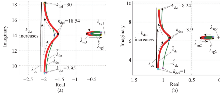
Fig. 5. Trajectories of eigenvalues and their estimates as k_{dci} increase from 1 to 30. (a) Trajectories of eigenvalues and their estimates as k_{dci} increase from 7.95 to 30. (b) Trajectories of eigenvalues and their estimates as k_{dci} increase from 1 to 8.24.
