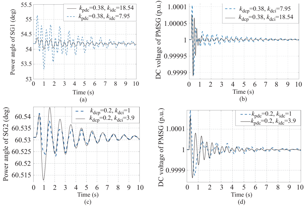
Fig. 6. Results of time domain simulation on the three-machine power system. (a) The difference between the power angle of SG1 when control parameter k_{dcp} = 0.38 , k_{dci} = 18.54 and k_{dcp} = 0.38 , k_{dci} = 7.95 . (b) The difference between the DC voltage of PMSG when control parameter k_{dcp} = 0.38 , k_{dci} = 18.54 and k_{dcp} = 0.38 , k_{dci} = 7.95 . (c) The difference between the power angle of SG2 when control parameter k_{dcp} = 0.2 , k_{dci} = 1 and k_{dcp} = 0.2 , k_{dci} = 3.9 . (d) The difference between the DC voltage of PMSG when control parameter k_{dcp} = 0.2 , k_{dci} = 1 and k_{dcp} = 0.2 , k_{dci} = 3.9 .
