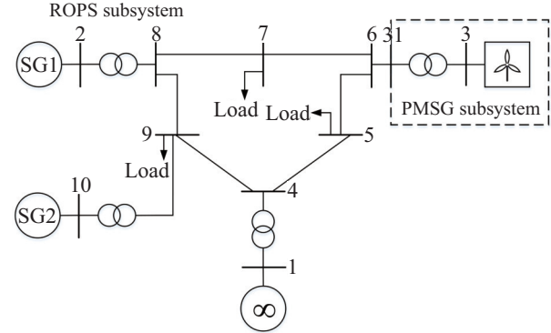
Fig. 4. Configuration of the three-machine power system.
